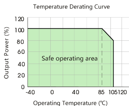
( Figure 1 ) Temperature curve
