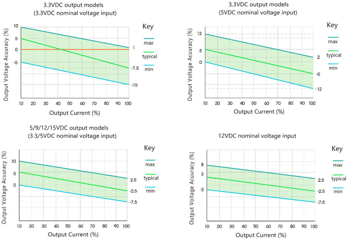
( Figure 2 ) Error envelope curve
