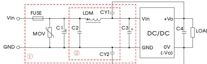
(Figure 3)EMC Recommended Circuit
